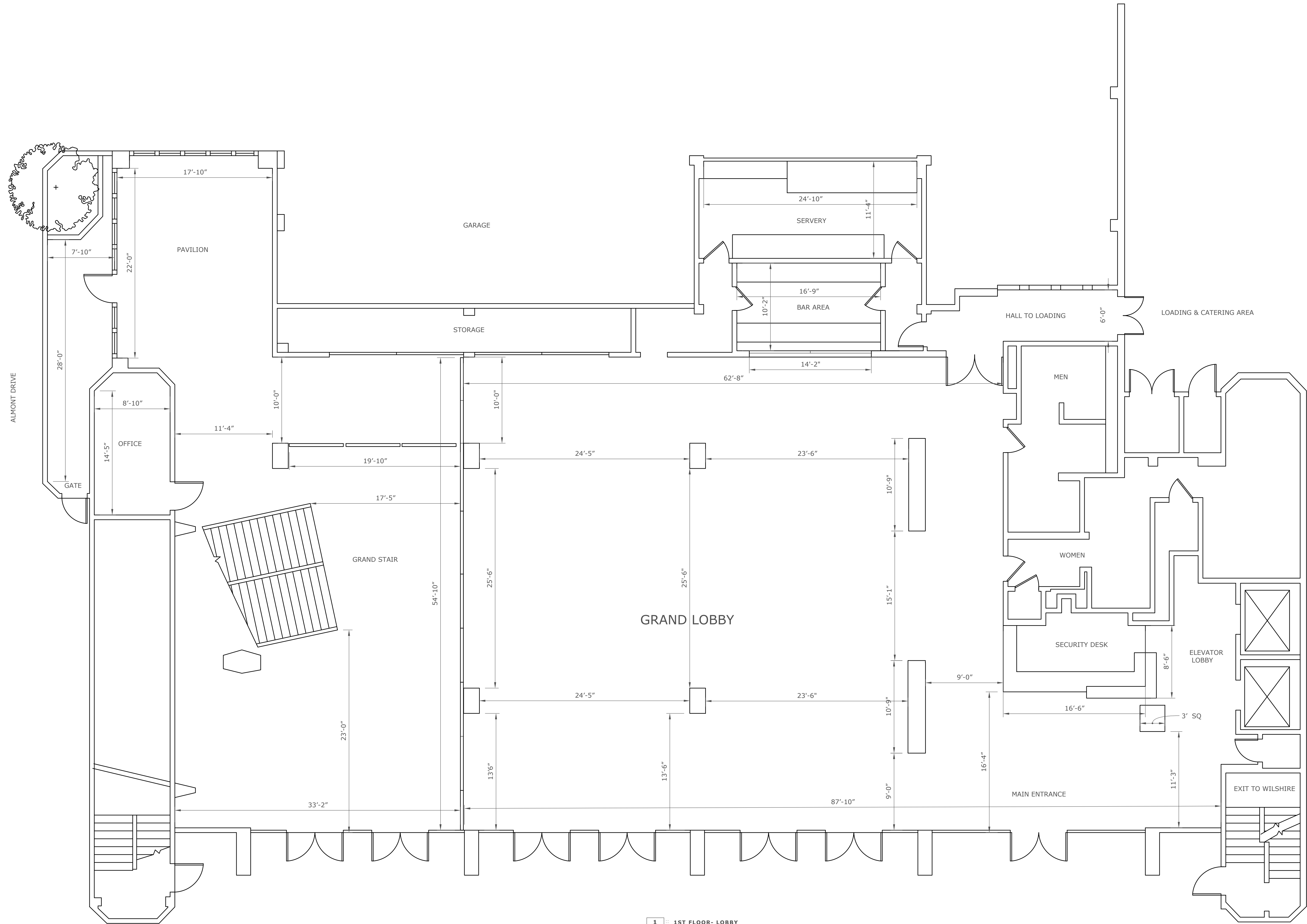
1 :: 1ST FLOOR- LOBBY 01 scale: 3/16" = 1'
